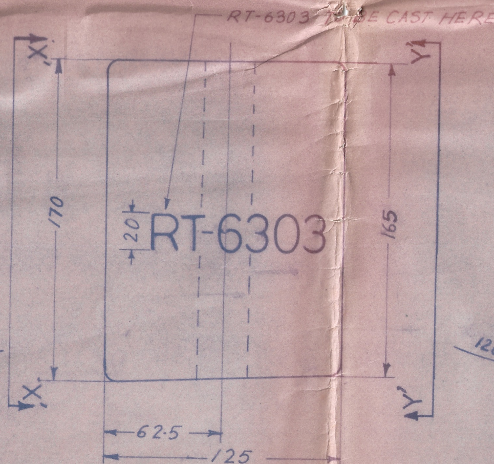
TOP PLAN
