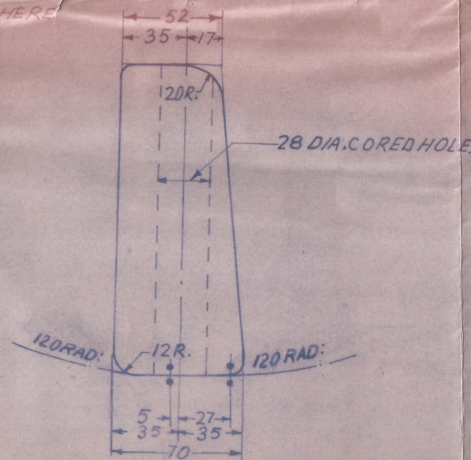
END ELEVATION Y'.Y'.
